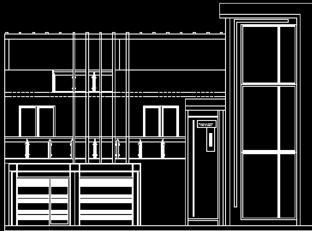
FACHADA PRINCIPAL
